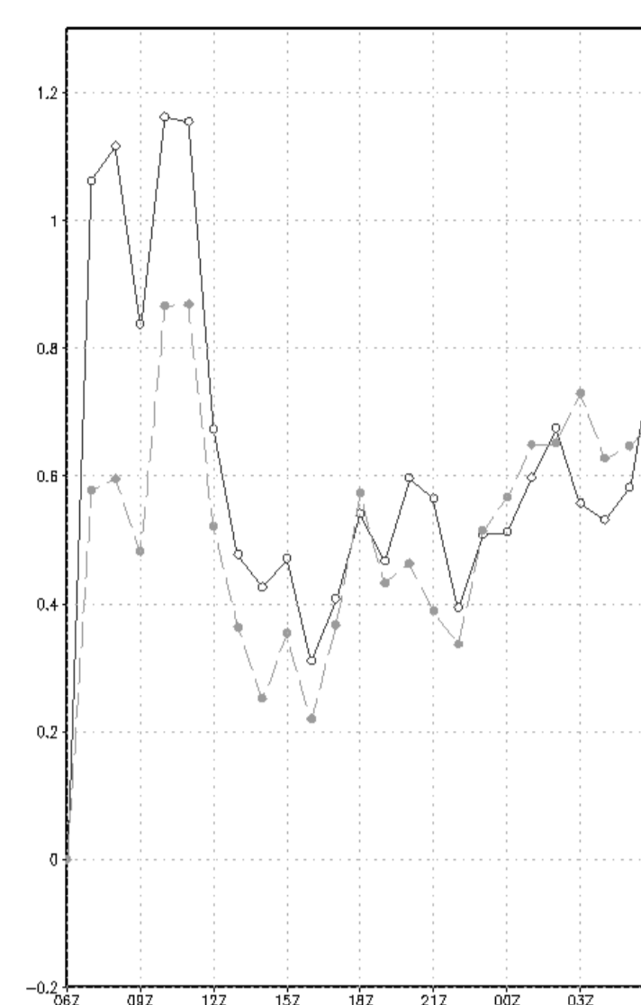
Figure 3. Temperature at 2m difference (vertical axis, °C) between control and modified runs. Solid line - LT10129II run and dashed line - LT10129I run.
