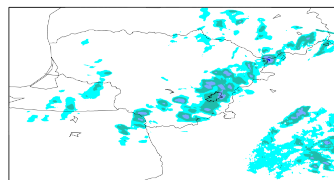
Figure 11. Precipitation at 2009-06-23 13 UTC, Control run.
