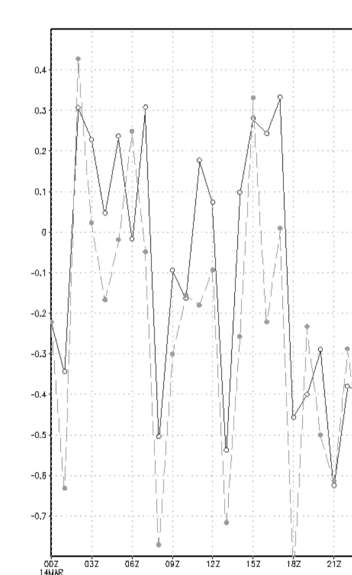
Figure 7. Wind speed at 10m difference (vertical axis, m/s) between control and modified runs. Solid line - LT30623II run and dashed line - LT30623I run.
