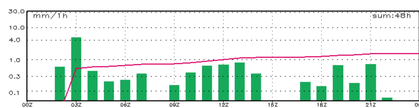
Figure 9. Precipitation at 2009-06-23, Control Run
