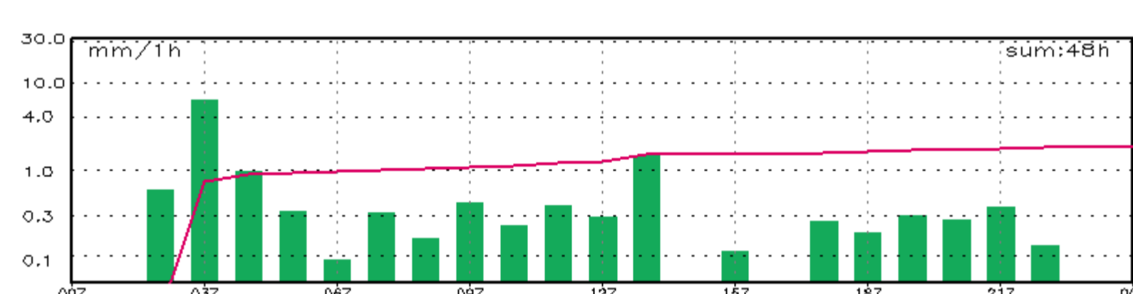
Figure 10. Precipitation at 2009-06-23, Modified Run
