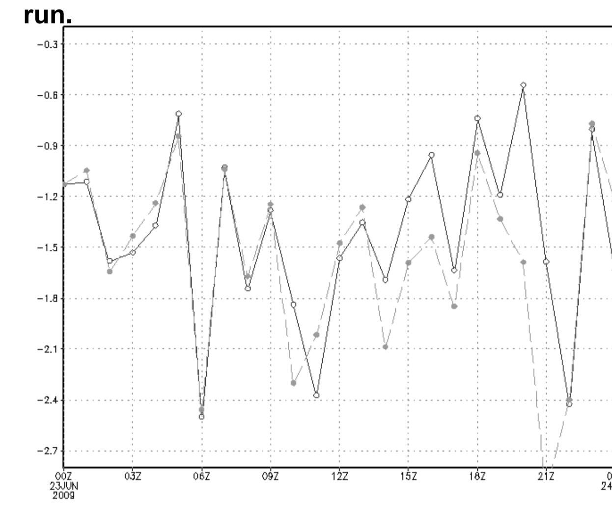
Figure 8. Wind speed at 10m difference (vertical axis, m/s) between control and modified runs. Solid line - LT30314II run and dashed line - LT30314I run.
