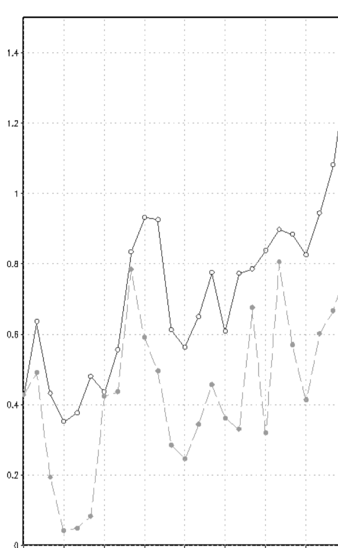
Figure 4. Temperature at 2m difference (vertical axis, °C) between control and modified runs. Solid line - LT30314II run and dashed line - LT30314I run.
