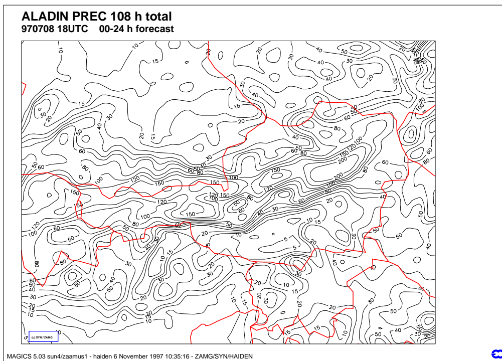
Figure 2: Precipitation totals predicted by ALADIN/LACE (00-24h forecast) during the 108h-period 97-07-04 06UTC to 97-07-08 18 UTC
