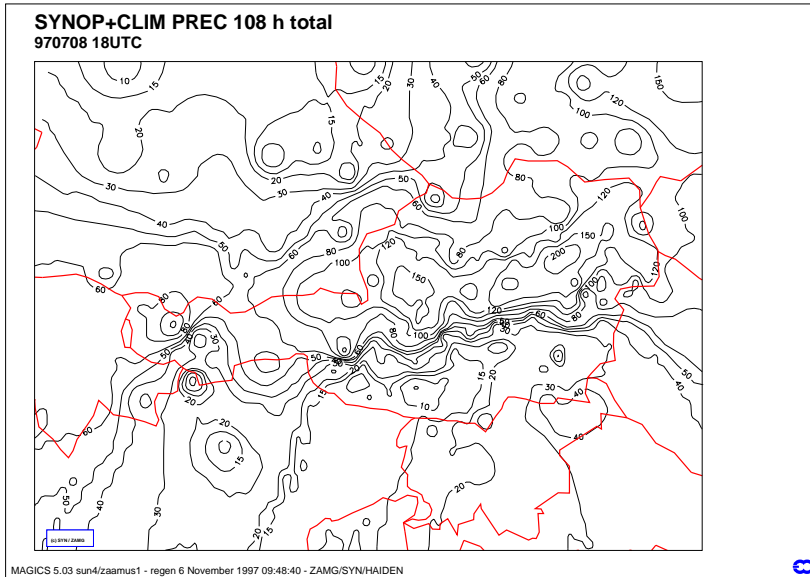
Figure 1: Observed precipitation totals of the 108h-period 97-07-04 06UTC to 97-07-08 18 UTC from synop and climate station reports, interpolated using an isotropic distance-weighting algorithm.
