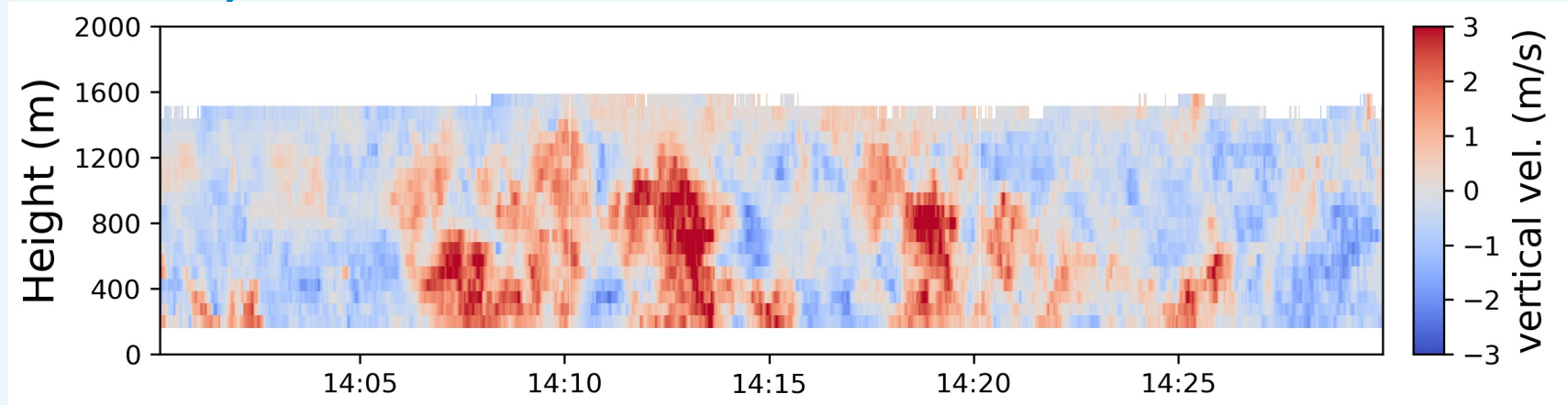
LES @ 19 m – coarsegrained to 100m
