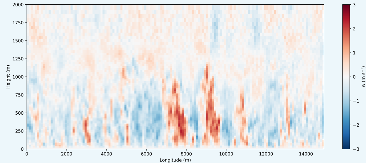
LES @ 19 m – coarsegrained to 100m
